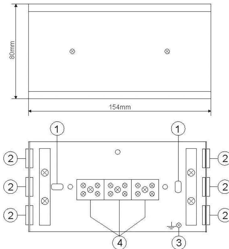
Fig.1. The junction box.
