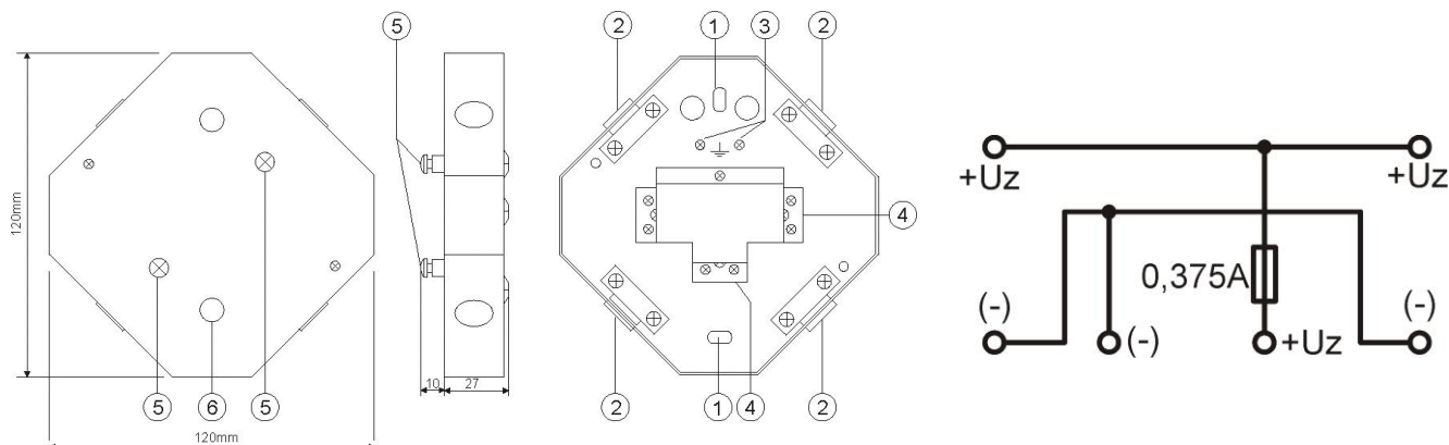
Fig.1. The junction box and wiring diagram.
